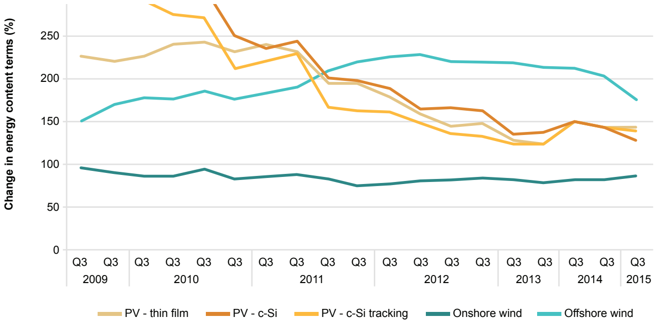
Figure 11. Global average levelised cost of electricity for wind and solar PV
